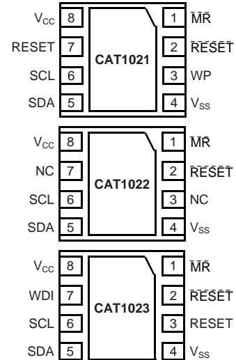
(Bottom View) TDFN Package: 3mm x 3mm 0.8mm maximum height - (ZD4)
